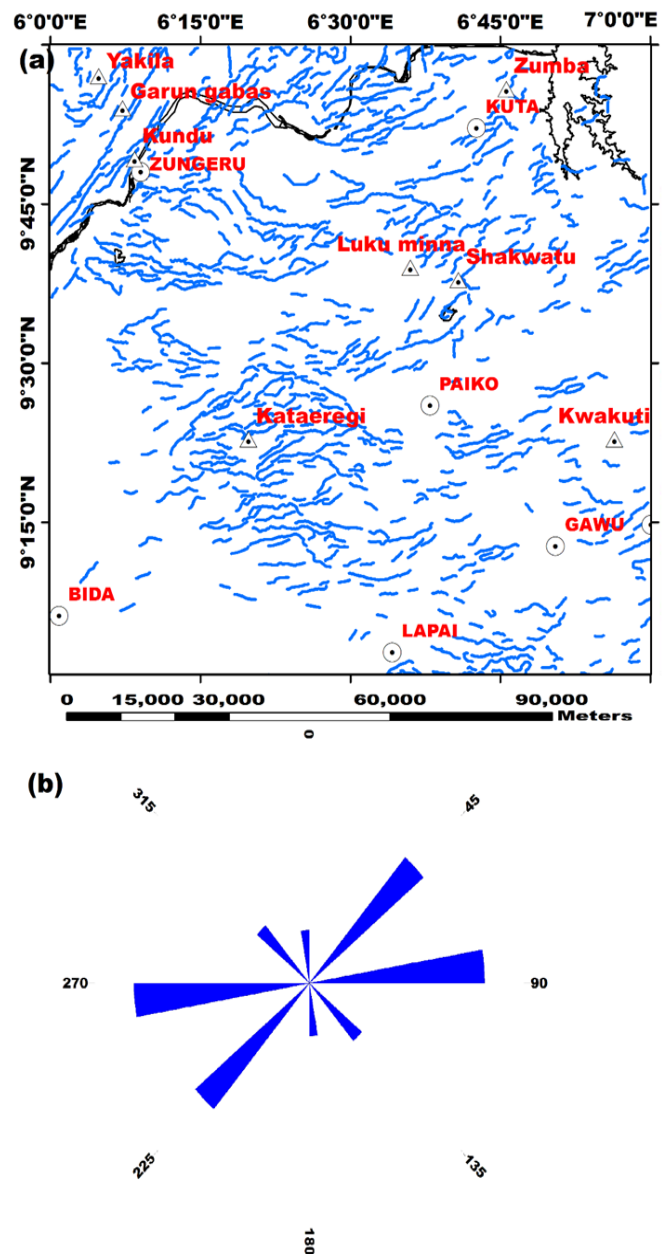
Figure 6: (a) Structural map of the study area produced from the extracted HP lineaments (b) Rose diagram produced from HP lineament
