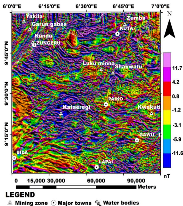
Figure 5: High pass map obtained from the reduced to pole anomaly of the study area
