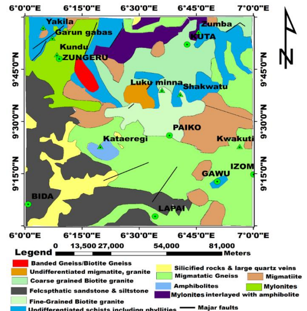
Figure 2: The geological map of the study area (modified after NGSA, 2010)
