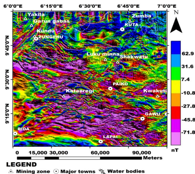
Figure 4: The reduced to pole anomaly map obtained from the total field anomaly
