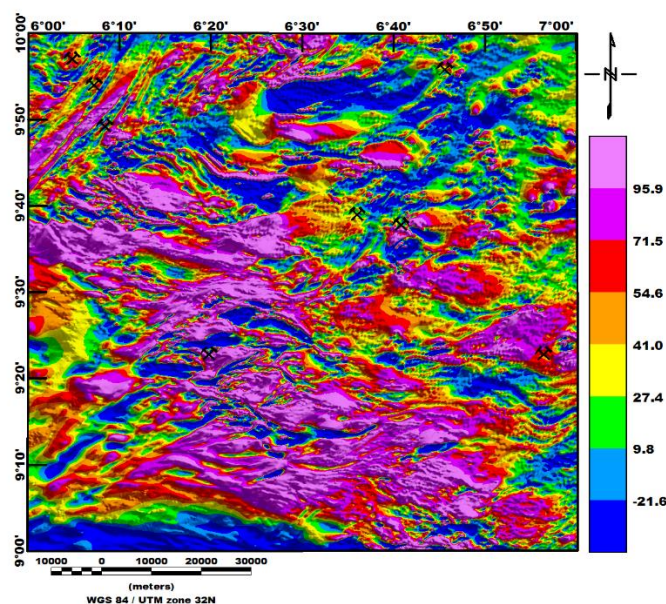
Figure 3a: Total field anomaly map of the study area
