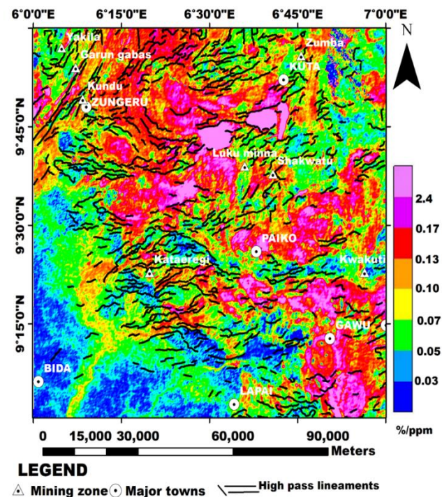
Figure 8: K/Th anomaly with superimposed HP lineaments map
